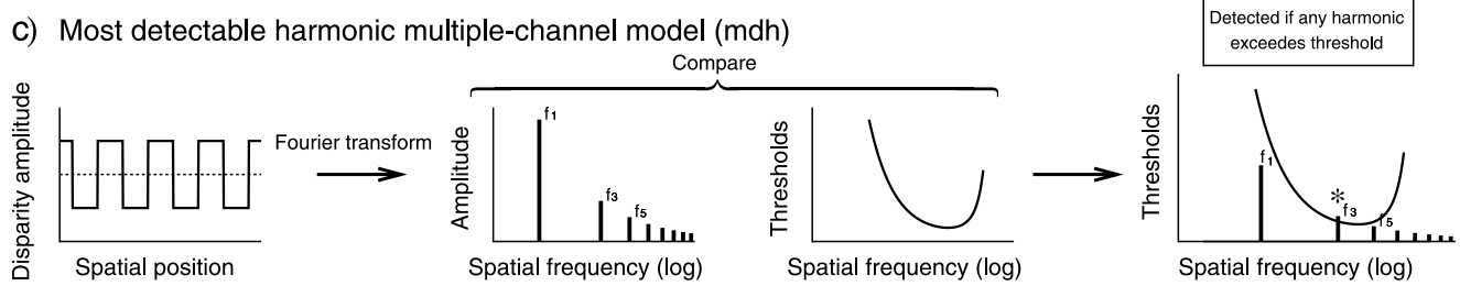
Figure 3. Schematic explaining the principles behind each model. The stimulus waveform is shown on the left of each row. In each case, the first step is to Fourier transform the waveform so as to obtain the amplitude of each component. In the single-channel models, this is then multiplied by the disparity sensitivity function (DSF) and inverse-transformed so as to produce a new waveform, which is the input convolved with a spatial linear operator whose Fourier transform corresponds to DSF. (a) The peak model postulates that the stimulus is detected if the peak amplitude of this filtered waveform exceeds some threshold value; (b) the rms model postulates that it is detected if its rms value exceeds some threshold. (c) The mdh model assumes that the stimulus is analyzed separately within each Fourier harmonic and is detected if any one of its harmonics exceeds the threshold needed to detect that harmonic in isolation.
